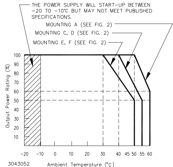
FIGURE 1. DERATING PLOT
