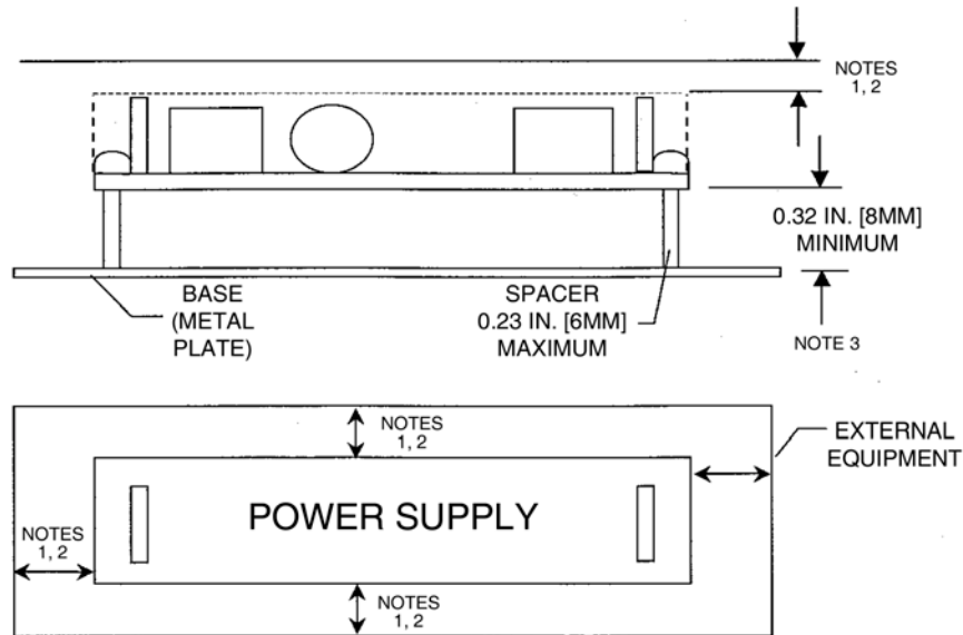
FIGURE 2. MOUNTING DIRECTION
